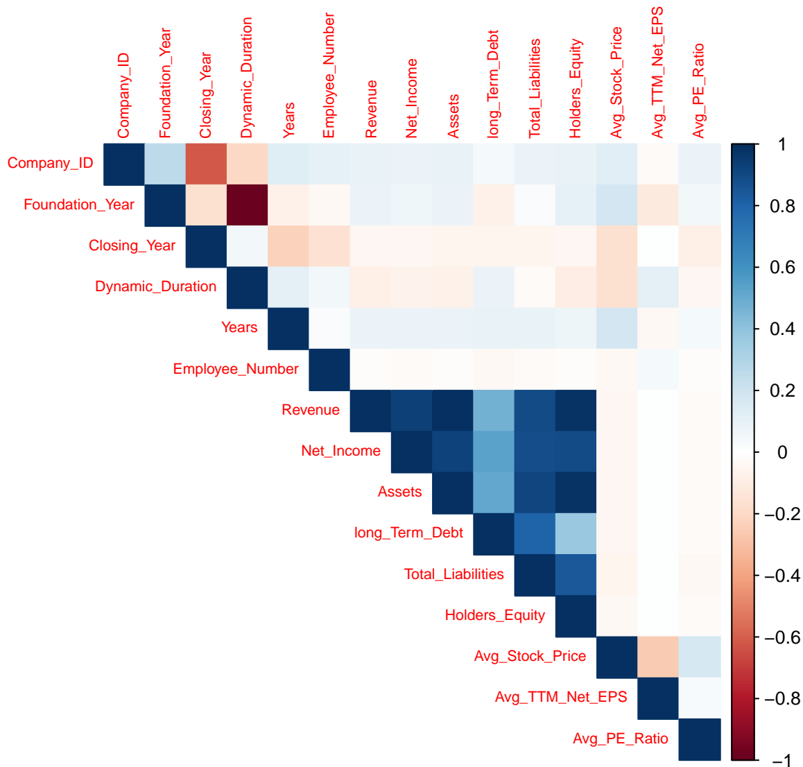
Correlation Matrix
